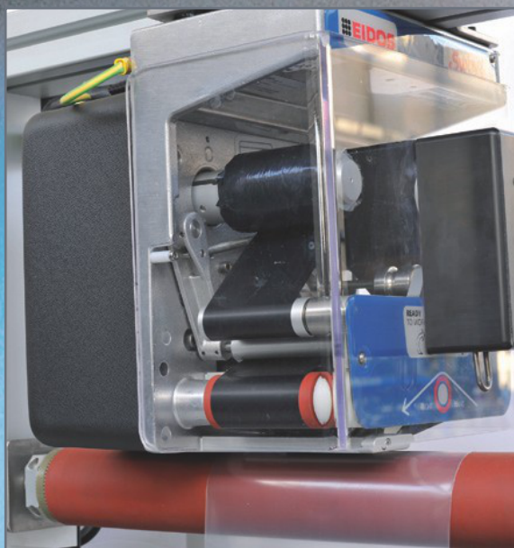
THERMO-TRANSFER-DRUCKER
